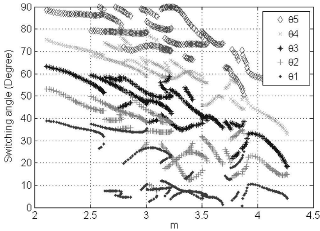
Fig. 4. Switching angles for harmonic elimination up to 17th.
