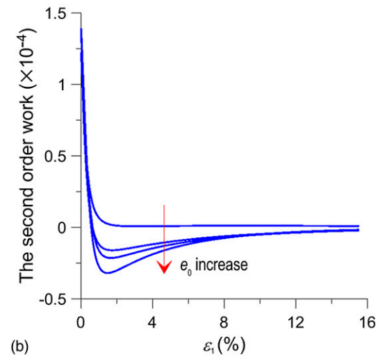
Fig. 11. Evolution of (a) determinant of the symmetric part of the elastoplastic modulus tensor; and (b) second-order work
