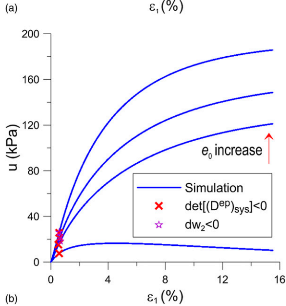
Fig. 10. Model prediction (experimental data after Chu and Wanatowski 2008): (a) stress-strain relationship; (b) evolution of pore-water pressure
